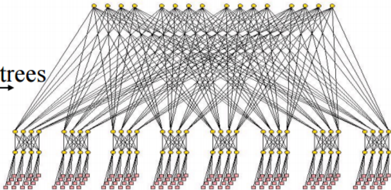
(b) A 128-way fat tree.
